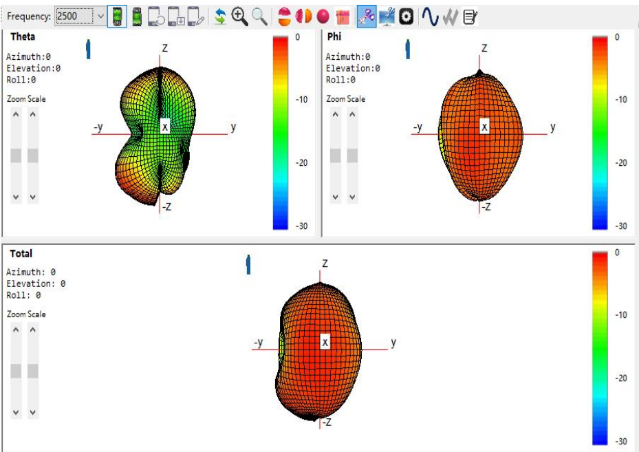
\phi = 0^\circ Plane XZ at 2500 MHz, Gain -0.60 dBi
