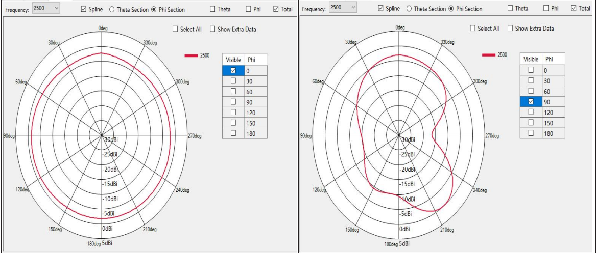
\phi = 0^\circ Plane XZ at 2500 MHz, Gain -0.60 dBi
